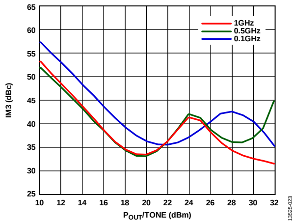
Figure 23. Output Third-Order Intermodulation (IM3) vs. P_{OUT}/TONE at V_{DD} = 28\text{ V}
