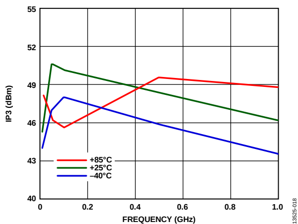
Figure 18. Output Third-Order Intercept (IP 3 ) vs. Frequency at Various Temperatures, P_{OUT}/Tone = 30\text{ dBm}
