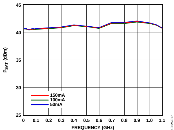
Figure 17. Saturated Output Power ( P_{SAT} ) vs. Frequency at Various Supply Currents
