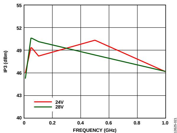
Figure 21. Output Third-Order Intercept (IP 3 ) vs. Frequency at Various Supply Voltages, P_{OUT}/Tone = 30\text{ dBm}
