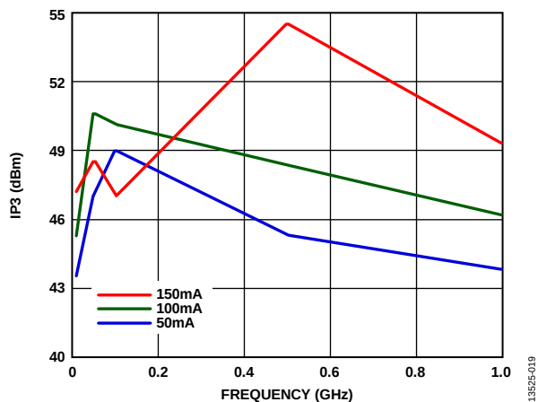
Figure 19. Output Third-Order Intercept (IP 3 ) vs. Frequency at Various Supply Currents, P_{OUT}/Tone = 30\text{ dB}
