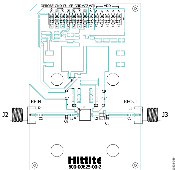
Figure 39. Evaluation Printed Circuit Board
