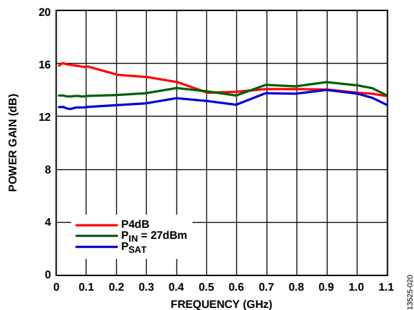
Figure 20. Power Gain vs. Frequency
