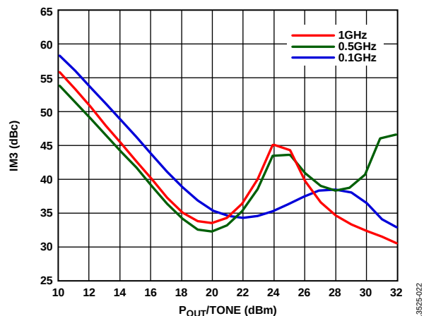
Figure 22. Output Third-Order Intermodulation (IM 3 ) vs. P_{OUT}/TONE at V_{DD} = 24\text{ V}
