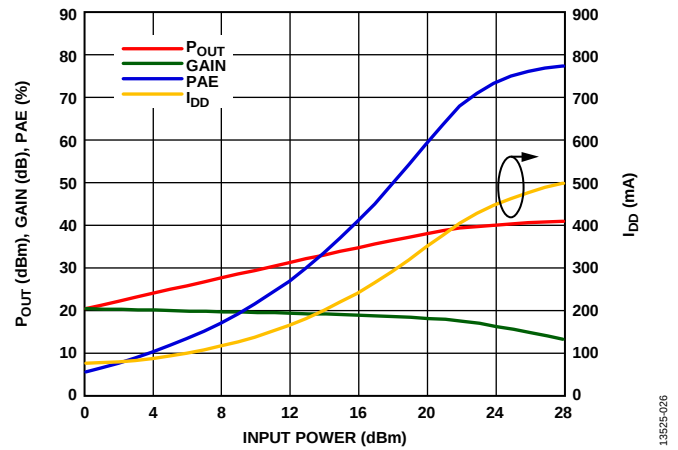
Figure 26. Power Output ( P_{OUT} ), GAIN, Power Added Efficiency (PAE), and Total Supply Current ( I_{DD} ) vs. Input Power at 0.1 GHz
