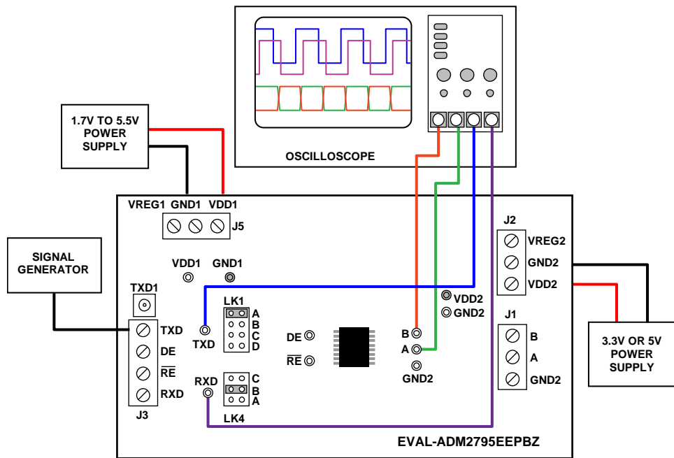
Figure 2. Basic Operation of the EVAL-ADM2795EEPBZ Evaluation Board for the ADM2795E-EP Robust 5 kV rms Isolated RS-485 Transceiver with Level 4 DO-160G and Full \pm 42 V Protection
