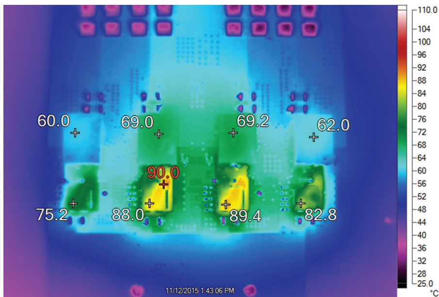
Figure 6. Thermal Picture of DC2291A, V_{IN} = 12V , V_O = 1.0V , I_O = 140A , F_{SW} = 450kHz , 400LFM Airflow, T_A = 25^\circ C
