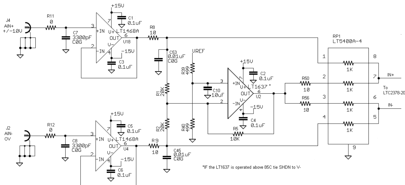
Figure 3. Pseudo-Differential Driver
