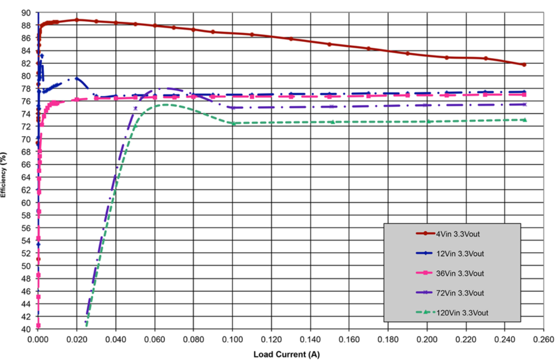
LTC3638 3.3V OUT Efficiency vs Load Current
