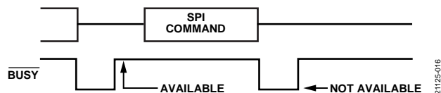
Figure 37. Busy Signal ( \overline{\text{BUSY}} ) Orientation After SPI Command
