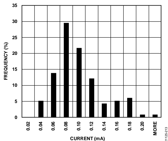
Figure 16. Sleep Mode Current Distribution at 3.0 V Supply
