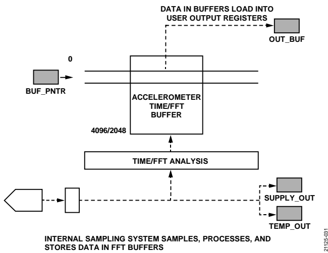
Figure 30. Data Buffer Structure and Operation
