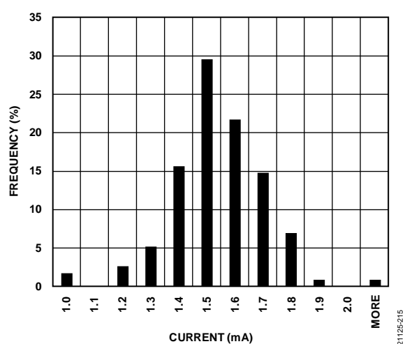
Figure 18. Sleep Mode Current Distribution at 3.6 V Supply
