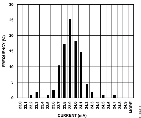
Figure 15. Operating Mode Current Distribution at 3.6 V Supply
