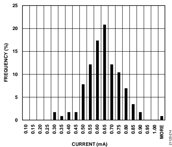
Figure 17. Sleep Mode Current Distribution at 3.3 V Supply
