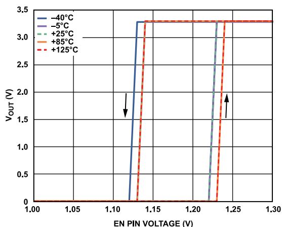
Figure 49. Typical VOUT Response to EN Pin Operation
