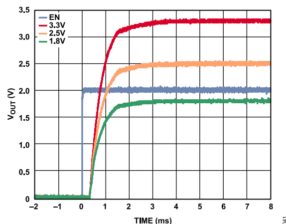
Figure 39. V_{OUT} Start-Up Time After V_{EN} Rising at Various Output Voltages, V_{IN} = 5.0\text{ V} , C_{BYP} = 1\text{ μF}
