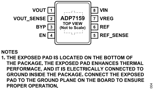
Figure 4. 8-Lead SOIC Pin Configuration
