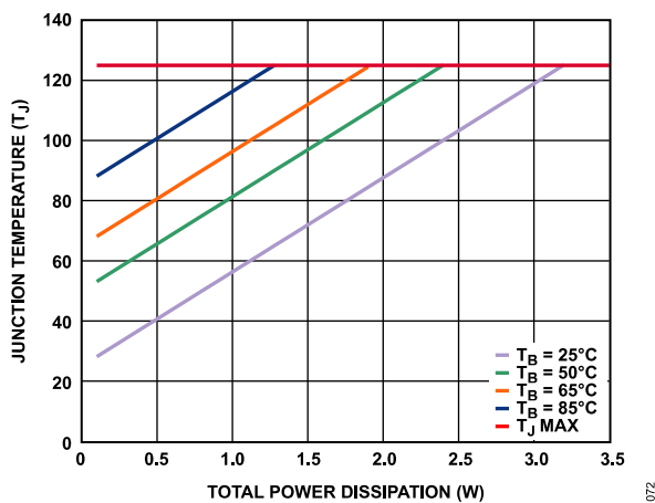
Figure 77. SOIC
