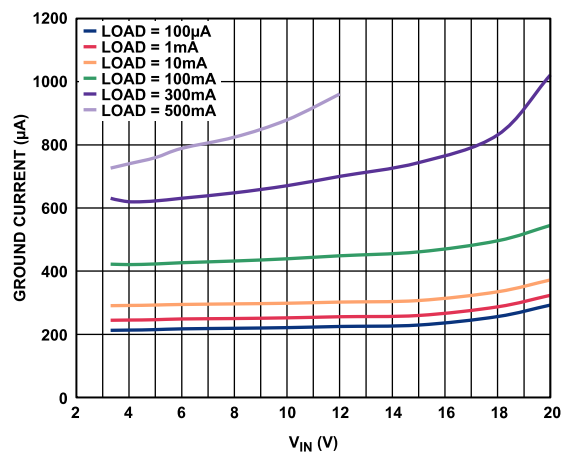
Figure 28. Ground Current ( I_{GND} ) vs. Input Voltage ( V_{IN} ), V_{OUT} = 1.8\text{ V}
