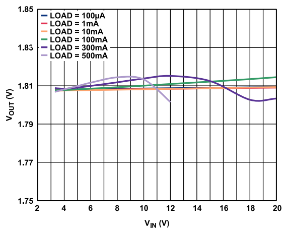
Figure 25. Output Voltage ( V_{OUT} ) vs. Input Voltage ( V_{IN} ), V_{OUT} = 1.8\text{ V}
