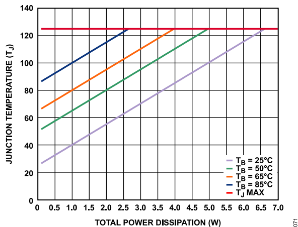
Figure 76. LFCSP
