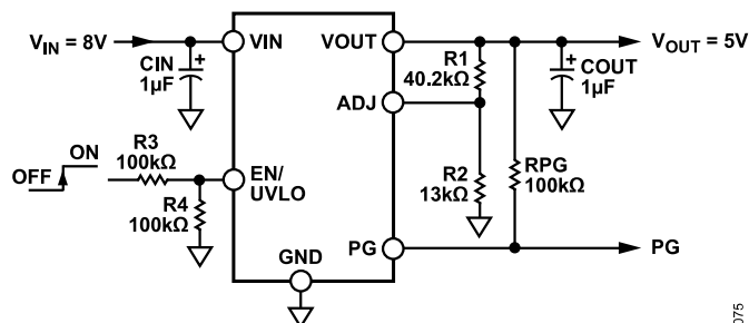
Figure 61. Typical Adjustable Output Voltage Application Schematic
