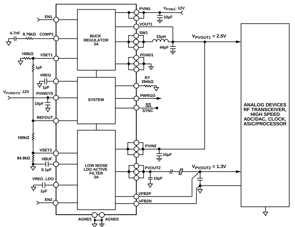
Figure 48. Independent Configuration (Dual Output)
