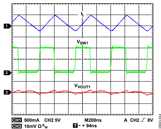
Figure 25. SW1 Waveform, V_{OUT1} = 5\text{ V} , I_{OUT1} = 100\text{ mA}
