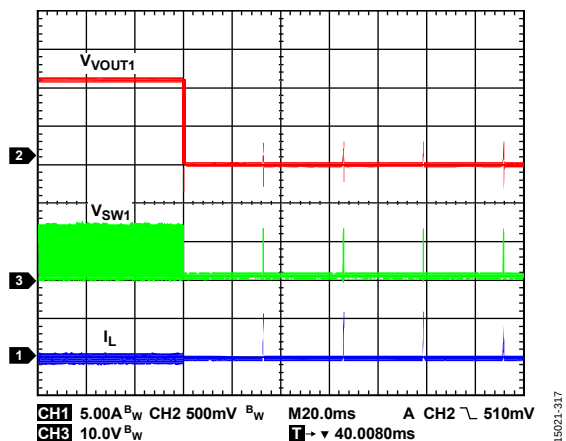
Figure 23. Entering Hiccup Mode ( V_{OUT1} is the Voltage of the VOUT1 Pin, and V_{SW1} is the Voltage of the SW1 Pin, and I_L is Inductor Current)
