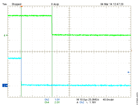
Figure 23. \overline{\text{RESET}} Timeout Delay With V_{CC} and V_{IN} Falling
