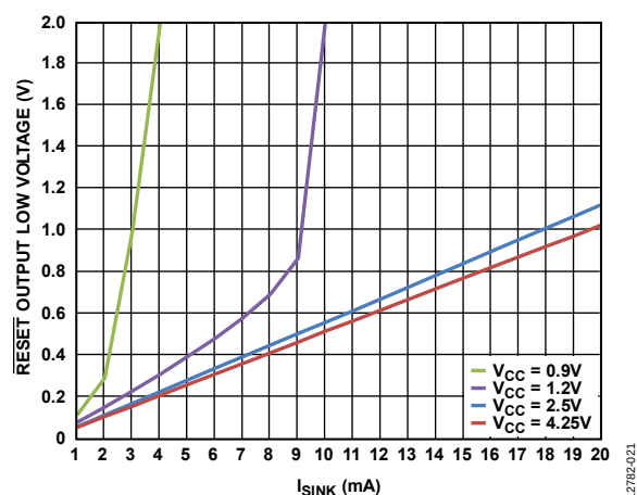
Figure 21. \overline{\text{RESET}} Output Low Voltage ( V_{RST\_OL} ) vs. Sink Current ( I_{SINK} )
