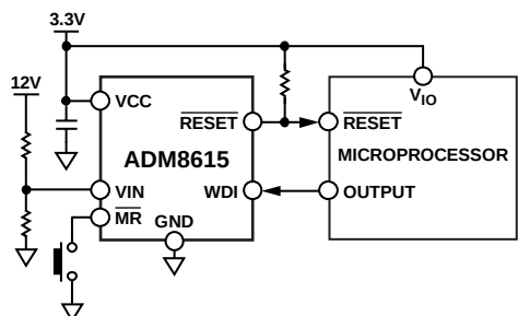
Figure 27. ADM8615 Typical Application Circuit
