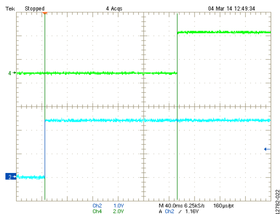
Figure 22. \overline{\text{RESET}} Timeout Delay With V_{CC} and V_{IN} Rising
