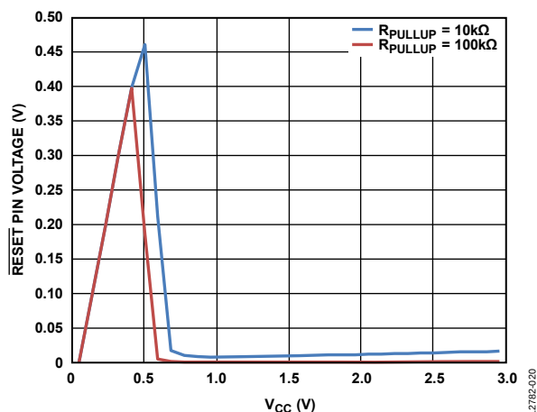
Figure 20. \overline{\text{RESET}} Pin Voltage vs. Voltage on V_{CC} (with the \overline{\text{RESET}} Pin Pulled Up to the V_{CC} Pin Through R_{PULLUP} )
