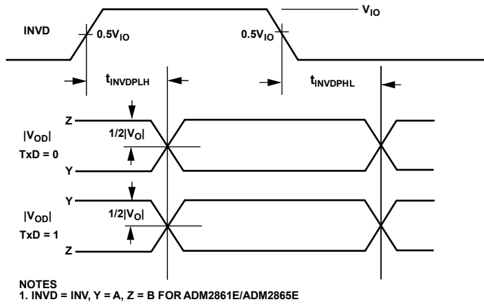
Figure 8. Driver Cable Invert Timing
