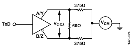
Figure 41. Driver Voltage Measurement over Common-Mode Range
