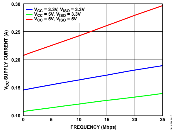
Figure 17. V CC Supply Current vs. Frequency, T A = 25°C, 54 Ω Load, 25 Mbps Models (ADM2865E and ADM2867E)
