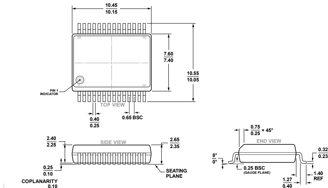
Figure 57. 28-Lead Standard Small Outline, Wide Body, with Finer Pitch [SOIC_W_FP] (RN-28-1)
