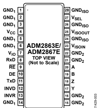
Figure 10. ADM2863E/ADM2867E Pin Configuration
