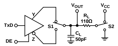
Figure 26. Driver Enable/Disable
