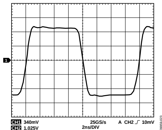
Figure 23. Large Signal Pulse Response, A_V = 15.5\text{ dB}
