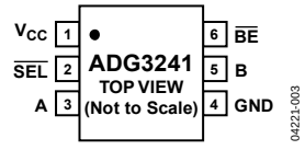
Figure 3. 6-Lead SOT-66
