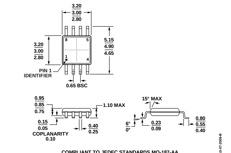
Figure 37. 8-Lead Mini Small Outline Package [MSOP] (RM-8)
