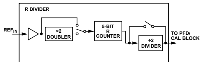
Figure 19. Reference Divider
