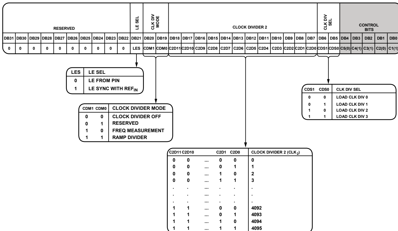
Figure 38. Register 13 (R13)
