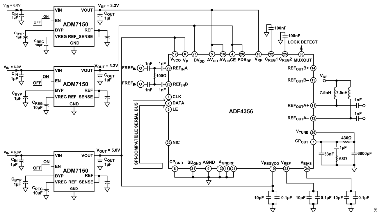
Figure 43. Power Supplies
