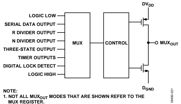
Figure 27. MUX_{OUT} Circuit
