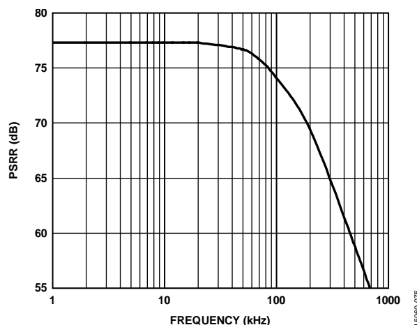
Figure 70. PSRR vs. Frequency
