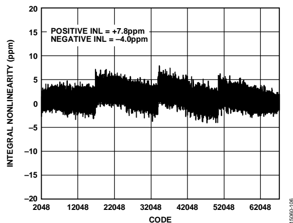
Figure 6. Integral Nonlinearity vs. Code, V_{+} = V_{DD} = 5\text{ V} , V_{-} = 0\text{ V} , REF = 3.3 V
