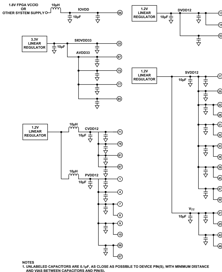
Figure 63. JESD204B Interface PCB Power Domain Recommendation
