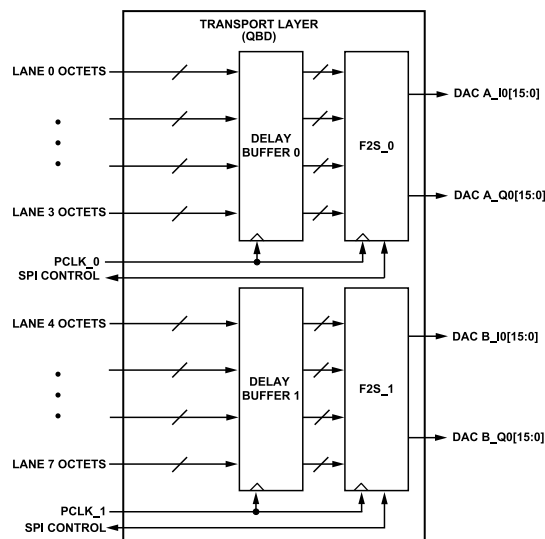
Figure 52. Transport Layer Block Diagram
