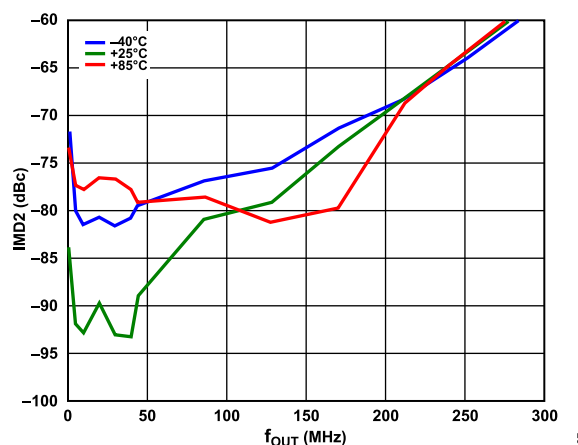
Figure 87. Post-Calibration IMD2 over Temperature, Calibrated at 25°C
