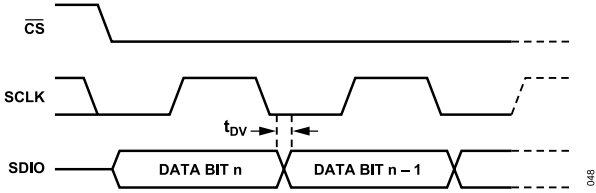
Figure 33. Timing Diagram for Serial Port Register Read
