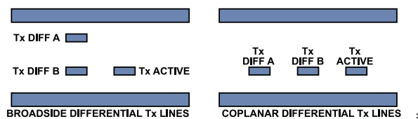
Figure 66. Broadside vs. Coplanar Differential Stripline Routing Techniques
