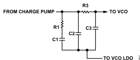
Figure 77. Loop Filter
