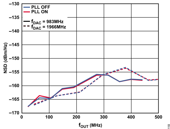
Figure 18. Single-Tone NSD (0 dBFS) vs. f_{OUT} , f_{DAC} = 983 MHz and 1966 MHz, PLL On and Off
