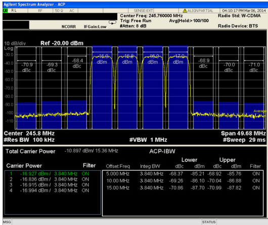
Figure 25. 4C WCDMA ACLR, f_{OUT} = 245 MHz, f_{DAC} = 1966 MHz, 4 \times Interpolation, PLL Frequency = 245 MHz
