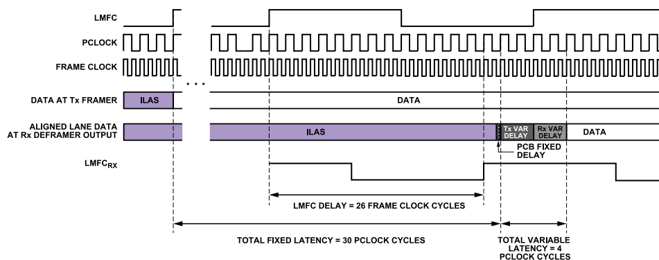
Figure 49. LMFC_DELAY Calculation Example
