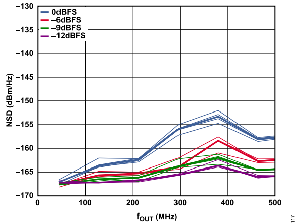
Figure 17. Single-Tone NSD vs. f_{OUT} over Digital Back Off, f_{DAC} = 1966 MHz
