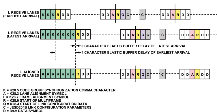
Figure 44. Lane Alignment During ILAS
