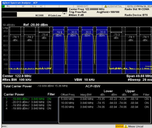
Figure 23. 4C WCDMA ACLR, f_{OUT} = 122 MHz, f_{DAC} = 983 MHz, 2 \times Interpolation, PLL Frequency = 122 MHz
