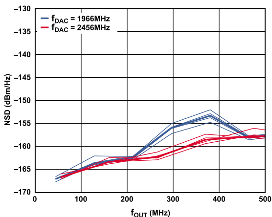
Figure 15. Single-Tone (0 dBFS) NSD vs. f_{OUT} , f_{DAC} = 1966 MHz and 2456 MHz
