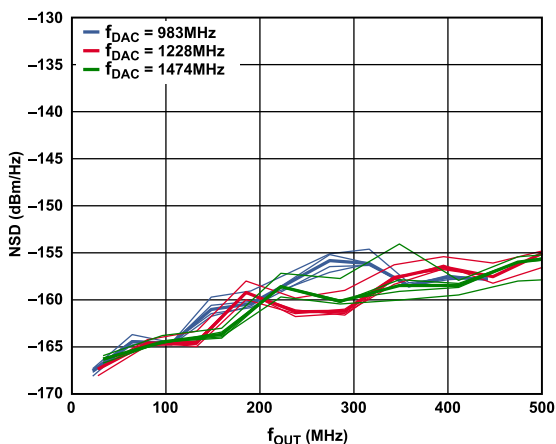
Figure 14. Single-Tone (0 dBFS) NSD vs. f_{OUT} , f_{DAC} = 983 MHz, 1228 MHz, and 1474 MHz
