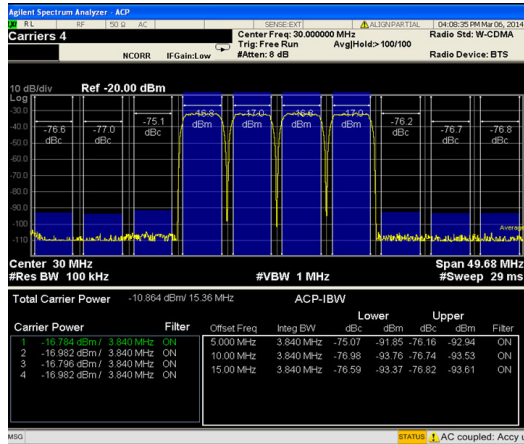
Figure 24. 4C WCDMA ACLR, f_{OUT} = 30 MHz, f_{DAC} = 1966 MHz, 4 \times Interpolation, PLL Frequency = 245 MHz
