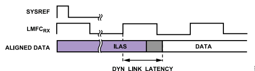
Figure 50. DYN_LINK_LATENCY Illustration
