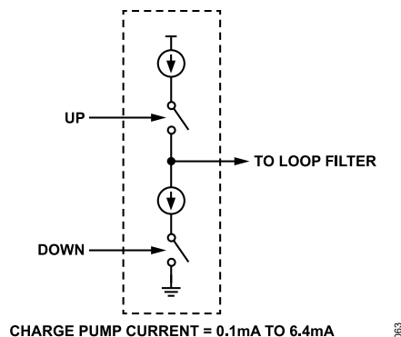
Figure 78. Charge Pump
