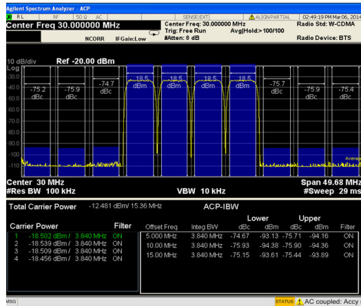
Figure 22. 4C WCDMA ACLR, f_{OUT} = 30 MHz, f_{DAC} = 983 MHz, 2 \times Interpolation, PLL Frequency = 122 MHz
