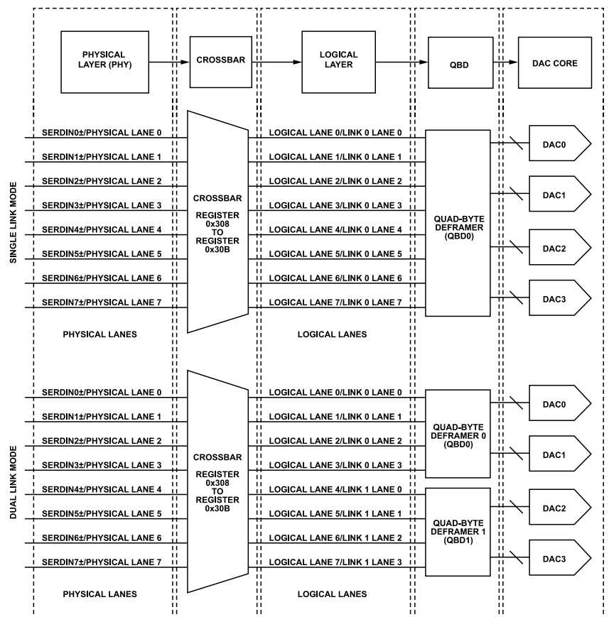
Figure 42. Link Mode Functional Diagram
