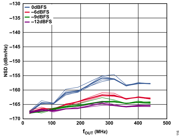
Figure 16. Single-Tone NSD vs. f_{OUT} over Digital Back Off, f_{DAC} = 983 MHz
