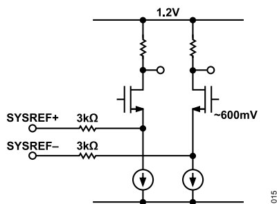
Figure 45. SYSREF \pm Input Circuit
