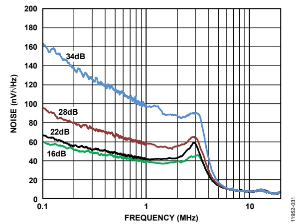
Figure 15. Short-Circuit Output Referred Noise vs. Frequency
