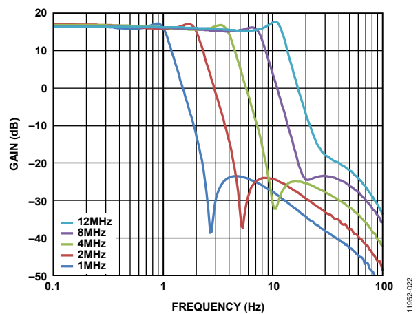
Figure 14. Filter Response
