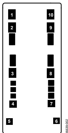
Figure 2. Metallization Diagram
