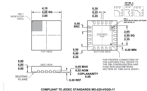
Figure 47. 20-Lead Lead Frame Chip Scale Package [LFCSP] 4 mm x 4 mm Body and 0.85 mm Package Height (CP-20-22) Dimensions shown in millimeters
