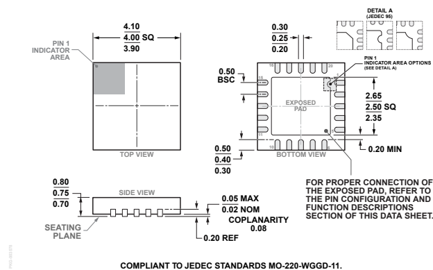
Figure 46. 20-Lead Lead Frame Chip Scale Package [LFCSP] 4 mm x 4 mm Body and 0.75 mm Package Height (CP-20-10) Dimensions shown in millimeters
