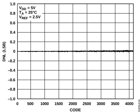
Figure 16. AD5681R DNL
