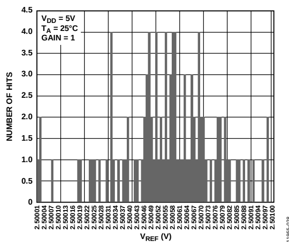
Figure 28. Reference Output Spread
