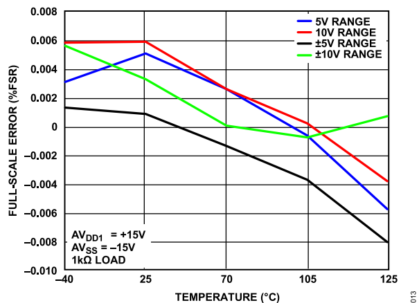
Figure 13. Full-Scale Error vs. Temperature
