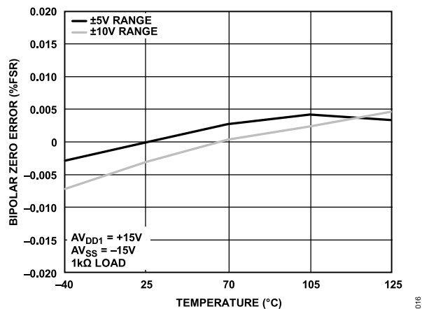
Figure 16. Bipolar Zero Error vs. Temperature
