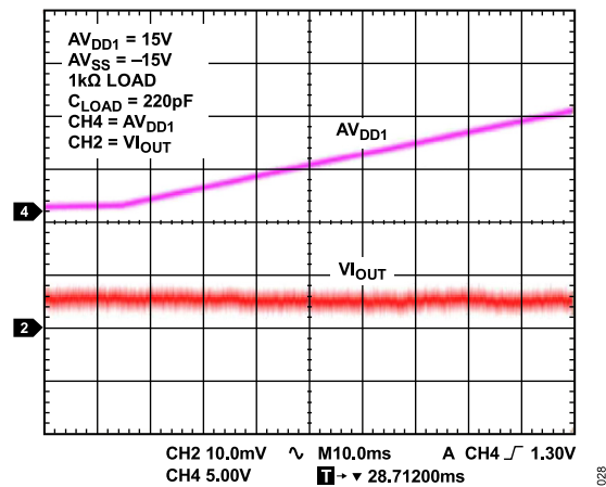
Figure 28. V_{\text{OUT}} vs. Time on Power Up
