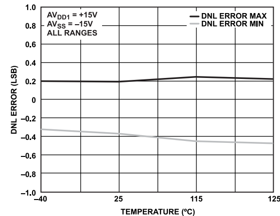
Figure 35. DNL Error vs. Temperature
