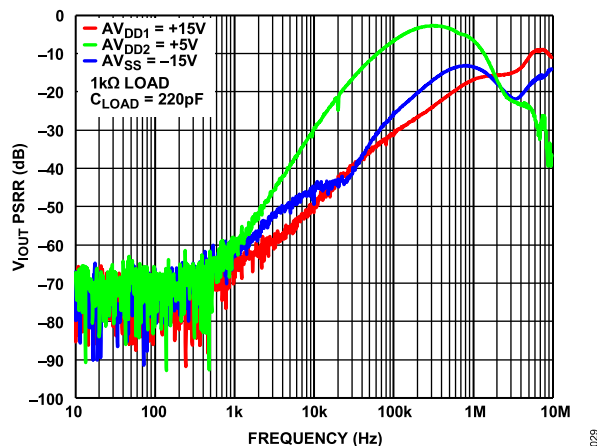
Figure 29. V_{\text{OUT}} PSRR vs. Frequency
