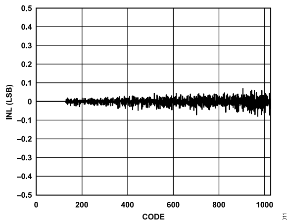
Figure 8. INL
