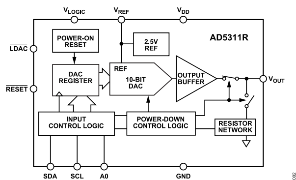
Figure 2. AD5311R
