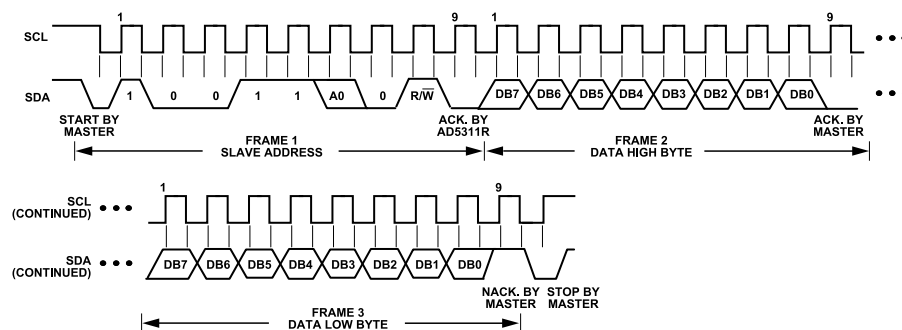
Figure 43. I²C Read Operation
