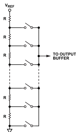
Figure 38. Simplified Resistor String Structure
