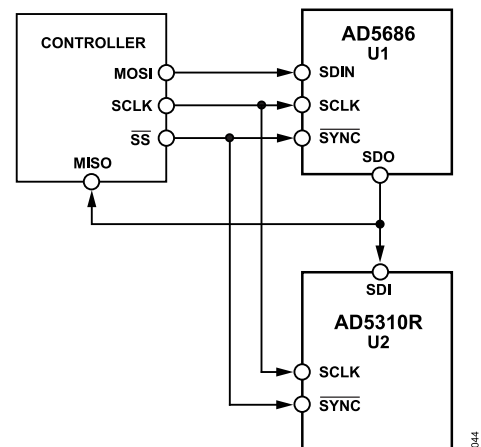
Figure 39. Daisy-Chain Connection
