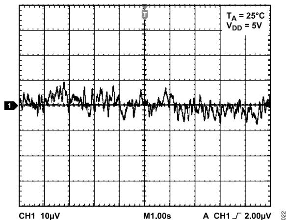
Figure 21. Internal Reference Noise, 0.1 Hz to 10 Hz
