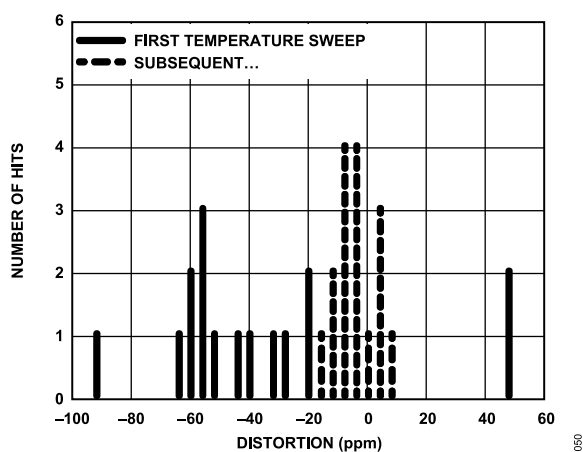
Figure 44. Thermal Hysteresis
