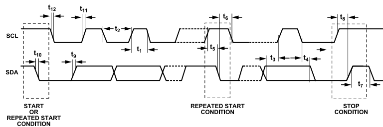
Figure 4. I²C Serial Interface Timing Diagram
