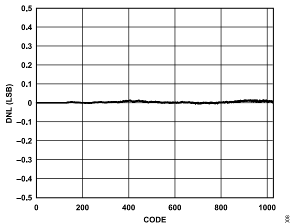
Figure 11. DNL
