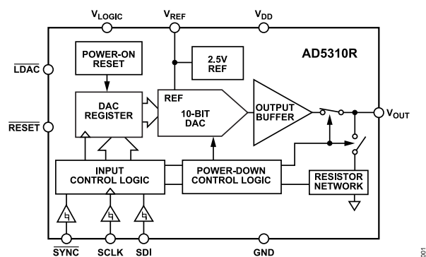
Figure 1. AD5310R
