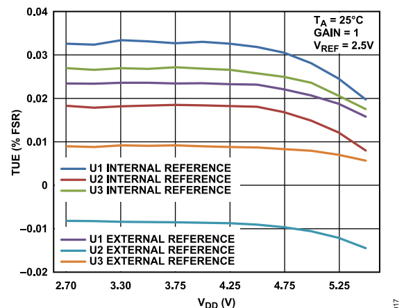
Figure 10. TUE vs. Supply, Gain = 1
