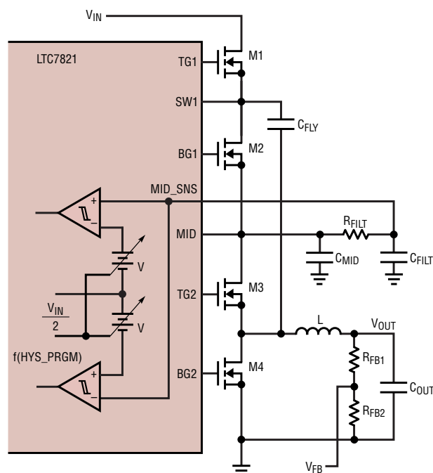
(19a) LTC7821 OUTPUT SETUP
