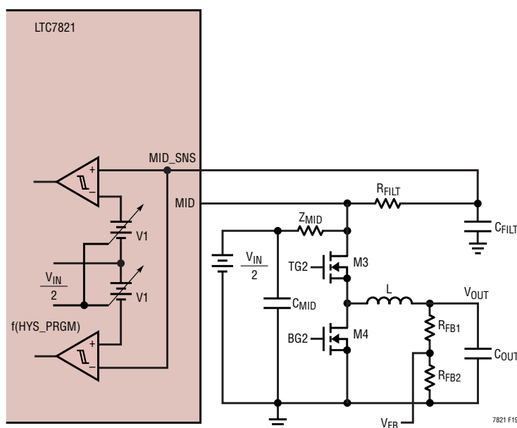
(19b) LTC7821 THEVENIN OUTPUT EQUIVALENT
