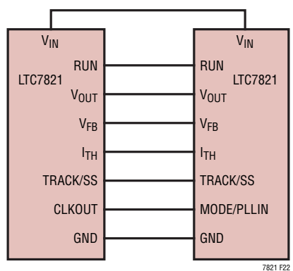
Figure 22. Connection of Key Signals of LTC7821 for Dual Phase Operation
