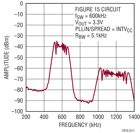
Output Voltage Frequency Spectrum (Spread Spectrum Enabled)
