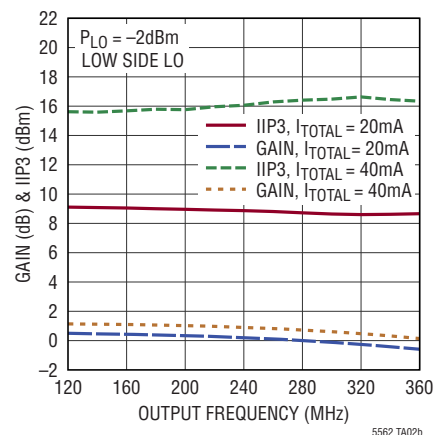
Conversion Gain and IIP3 vs Output Frequency, f_N = 3.6\text{GHz}
