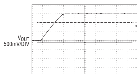
12V to 1.5V Full-Load Start-Up
