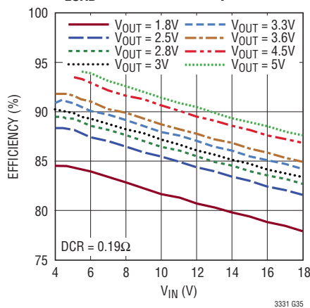
Buck Efficiency vs V_{IN} for I_{LOAD} = 100\text{mA} , L = 22\mu\text{H}
