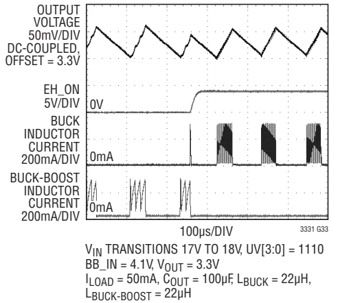
Prioritizer Buck-Boost to Buck Transition
