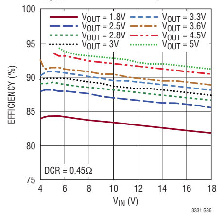
Buck Efficiency vs V_{IN} for I_{LOAD} = 100\text{mA} , L = 100\mu\text{H}
