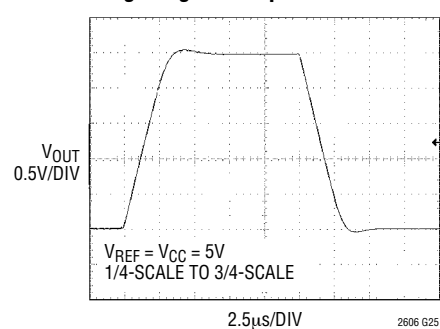
Large-Signal Response
