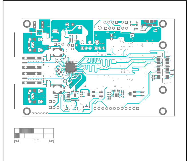
MAX96716/MAX96792 EV Kit Component Placement Guide— Top
