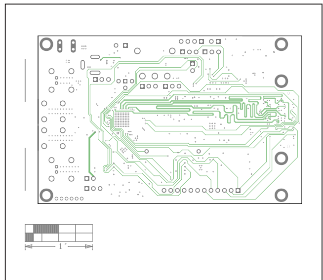
MAX96716/MAX96792 EV Kit Component Placement Guide— L3_SIG
