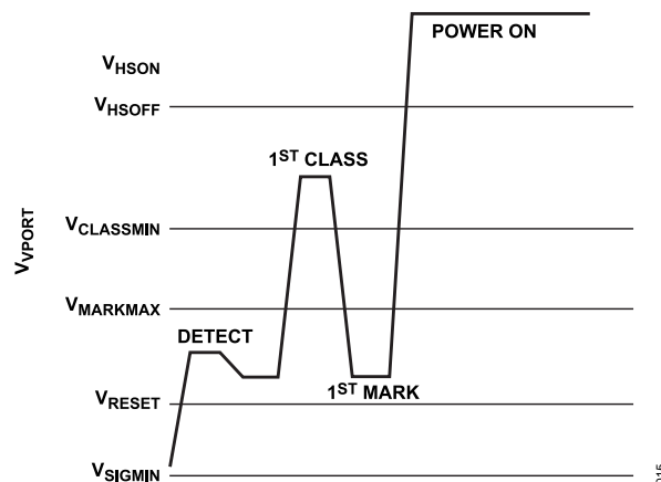
Figure 15. Type 3 or 4 PSE, Detection and 1-Event Class Sequence
