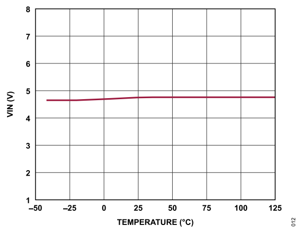
Figure 12. VIN Pin Reset Threshold
