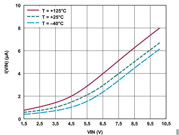
Figure 9. VIN Pin Detection Current
