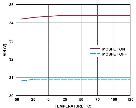
Figure 10. V_{ON} and V_{OFF} Thresholds
