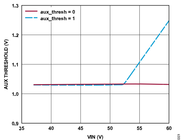
Figure 3. AUX Pin Thresholds
