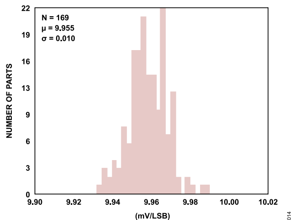
Figure 14. Voltage Readback LSB Weight
