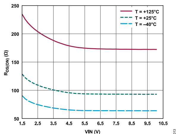
Figure 13. RSIG Pin Pull-down Resistance
