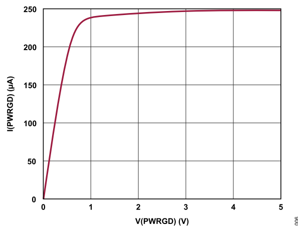
Figure 6. PWRGD Pin Pull-down Current
