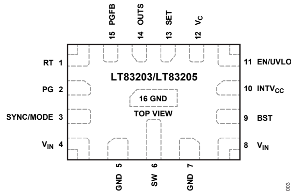
LFCSP PACKAGE
