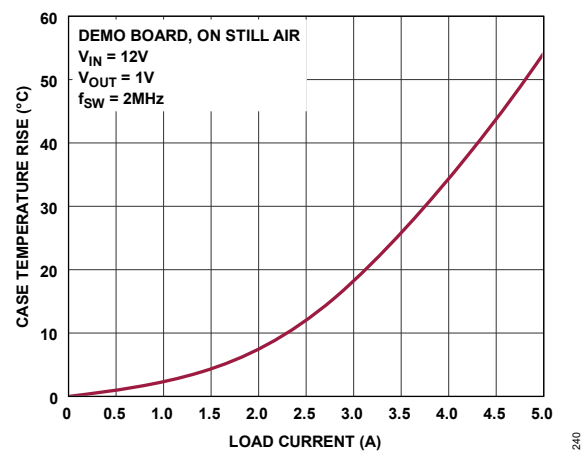
Figure 43. LT83203/LT83205 Case Temperature Rise
