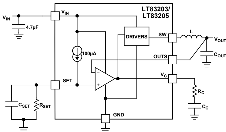
Figure 52. Adjustable Reference for Error Amplifier
