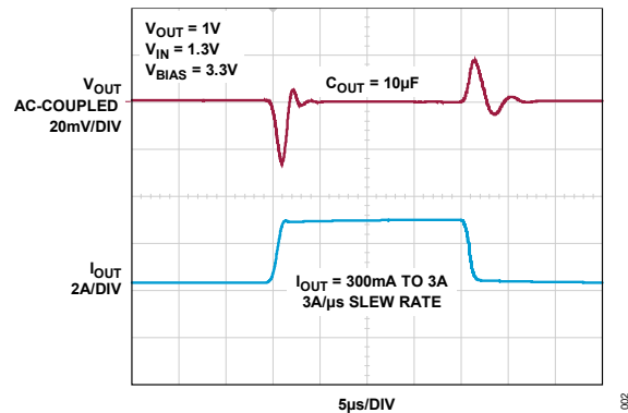
Figure 2. Transient Response
