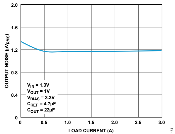
Figure 54. Integrated RMS Output Noise (10Hz to 100kHz)
