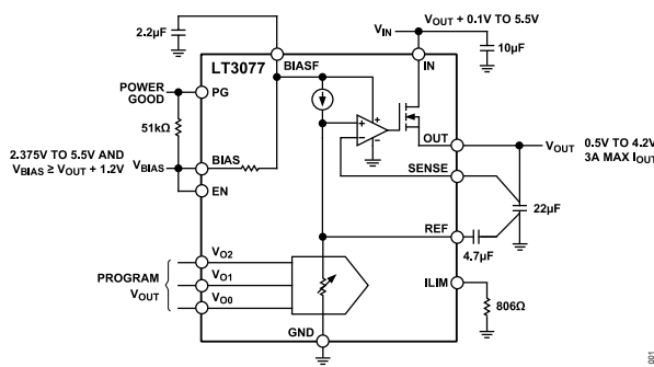
Figure 1. Simplified Application Diagram
