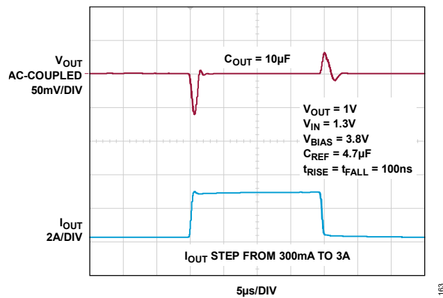
Figure 63. Load Transient
