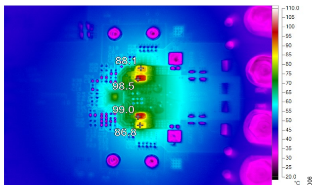
Figure 7. Thermal Performance with 24V Input, 48V Output, and 16.5A Load. No heatsink or airflow. The hottest component on EVAL-LTC7892-BZ stays under 100^{\circ}\text{C} .
