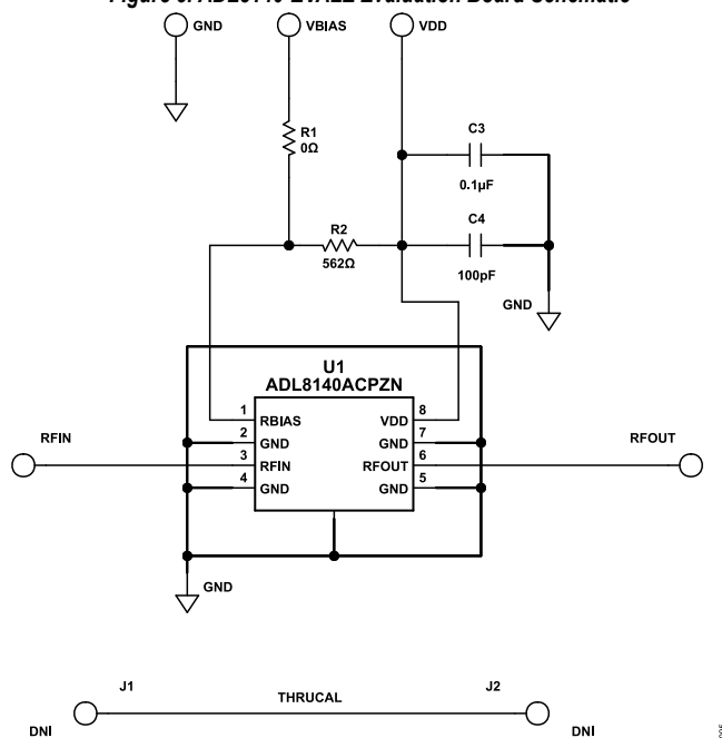
Figure 5. ADL8140-EVALZ Evaluation Board Schematic
