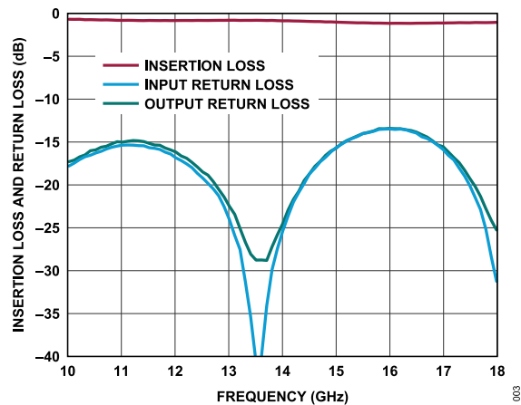
Figure 3. Insertion Loss and Return Loss of the Through Calibration Path, 10 GHz to 18 GHz
