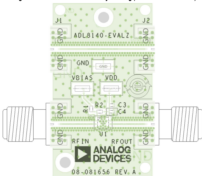
Figure 6. ADL8140-EVALZ Assembly Drawing (J1 and J2 Not Installed)
