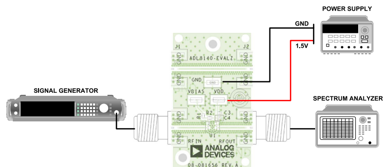
Figure 4. ADL8140-EVALZ Operating Block Diagram
