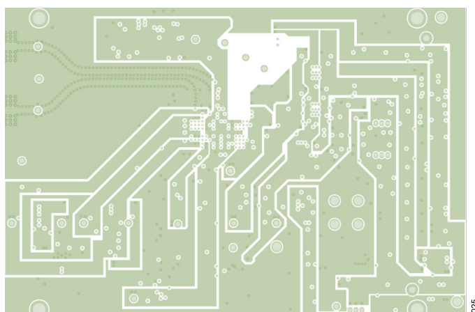
Figure 24. EVAL-ADAQ4216-FMCZ, Power Layer 3
