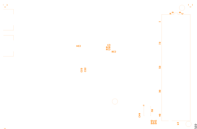
Figure 21. EVAL-ADAQ4216-FMCZ Silkscreen, Bottom Layer
