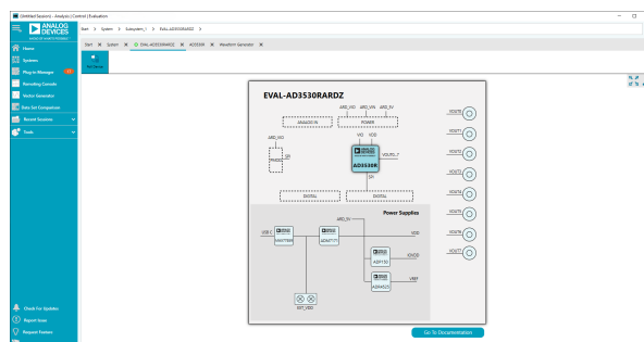
Figure 1. Board View of the EVAL-AD3530RARDZ
