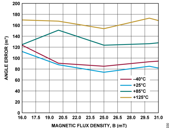
Figure 9. Angle Measurement Accuracy vs. Operating Magnetic Flux Density at 3.3 V
