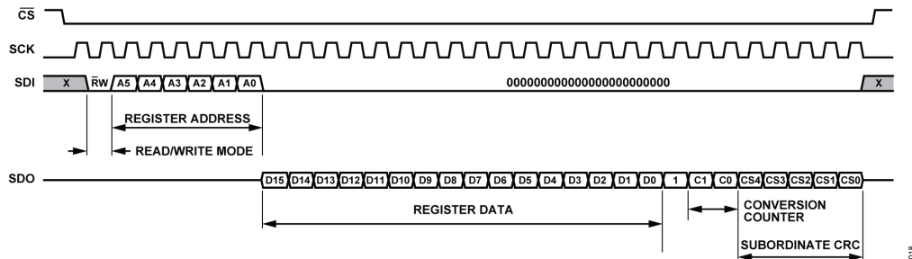
Figure 18. SPI Register Read Operation
