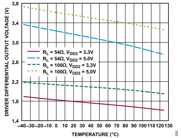
Figure 30. Driver Differential Output Voltage vs. Temperature
