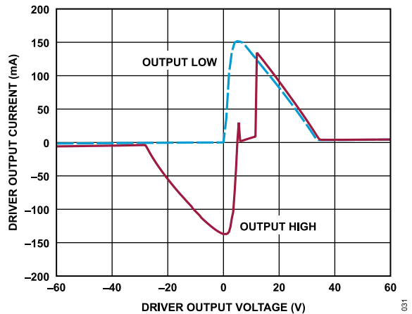
Figure 31. Driver Output Current vs. Driver Output Voltage
