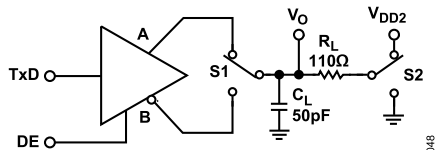
Figure 48. Driver Enable or Disable Time Measurement
