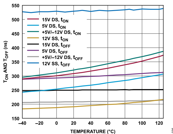
Figure 35. t_{ON} , t_{OFF} Times vs. Temperature
