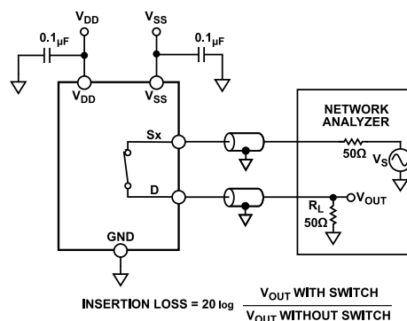
Figure 43. Bandwidth
