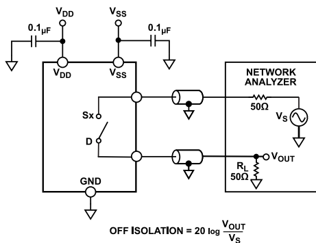
Figure 39. Off Isolation
