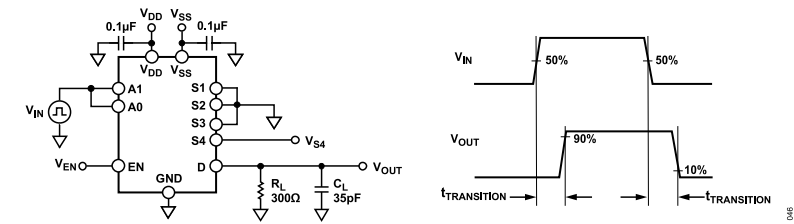
Figure 46. Switching Times
