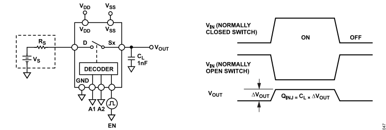
Figure 47. Charge Injection
