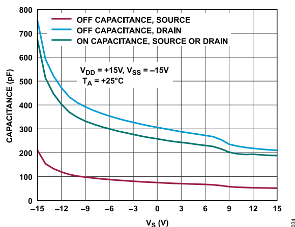
Figure 34. Capacitance vs. V_S , ±15V Dual Supply
