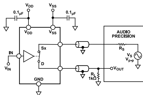
Figure 42. THD + Noise
