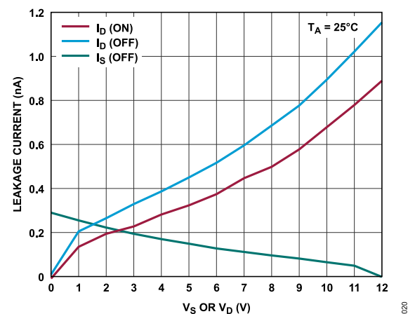
Figure 20. Leakage Currents as a Function of V_S(V_D) , 25°C, 12V Single Supply
