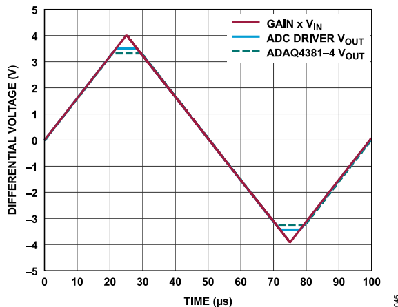
Figure 45. Output Overdrive Recovery, Gain = 0.6
