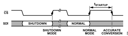
Figure 6. Shutdown Mode to Normal Mode Timing
