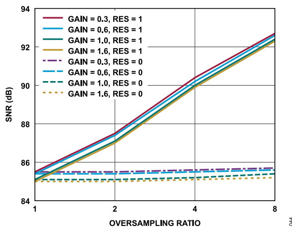
Figure 44. SNR vs. Rolling Average Oversampling, f_{IN} = 1 kHz
