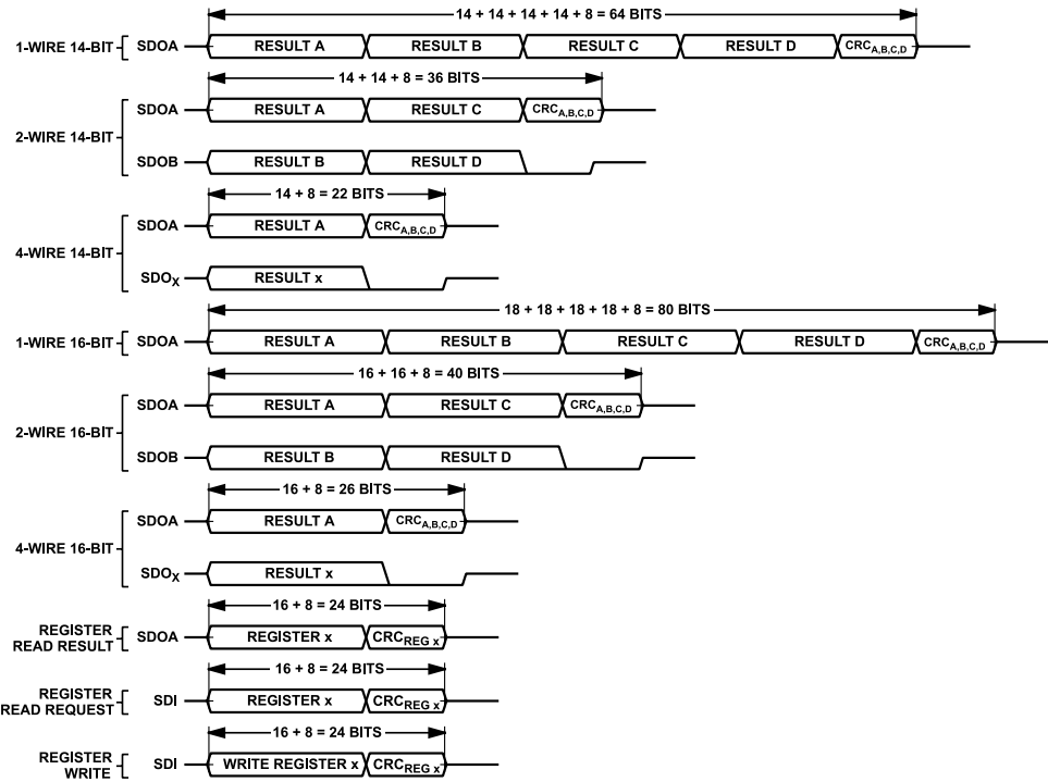
Figure 78. CRC Operation
