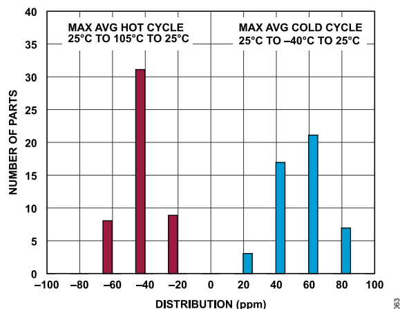
Figure 64. Reference Output Voltage Hysteresis at Half Cycles
