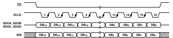
Figure 68. Resolution Boost
