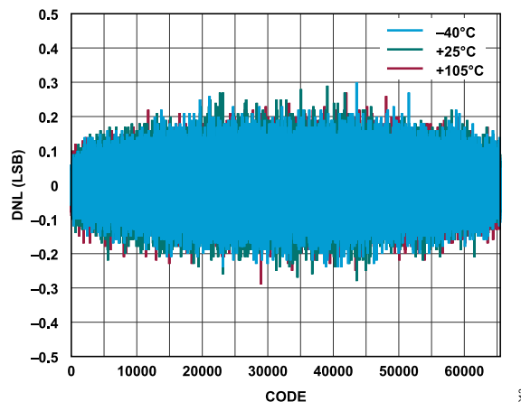
Figure 13. DNL vs. Code for Various Temperature, Gain = 1.0
