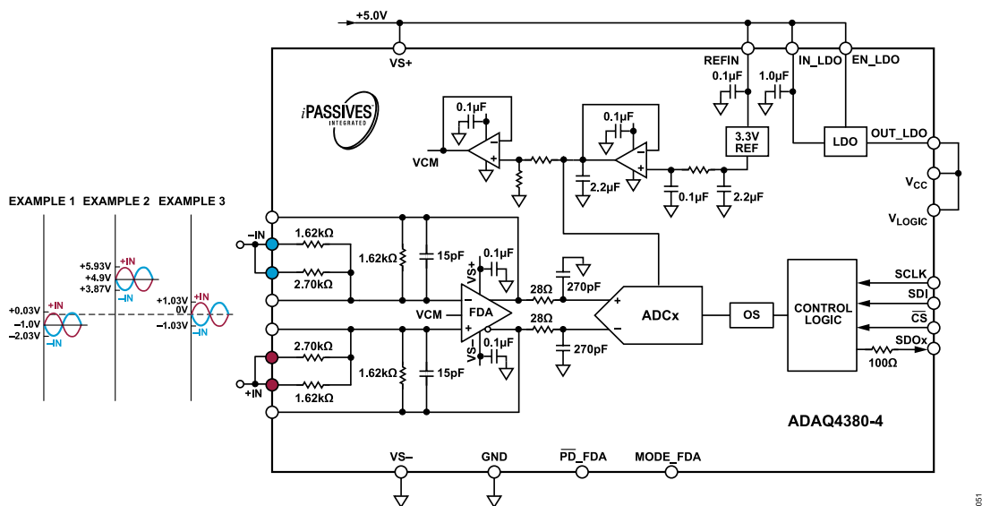
Figure 51. Fully Differential Input Configuration with Gain = 1.6, \pm 2.06\text{ V} Input, V_S = 5\text{ V}
