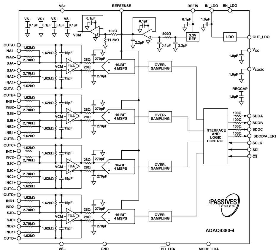
Figure 46. ADAQ4380-4 μModule Simplified Block Diagram
