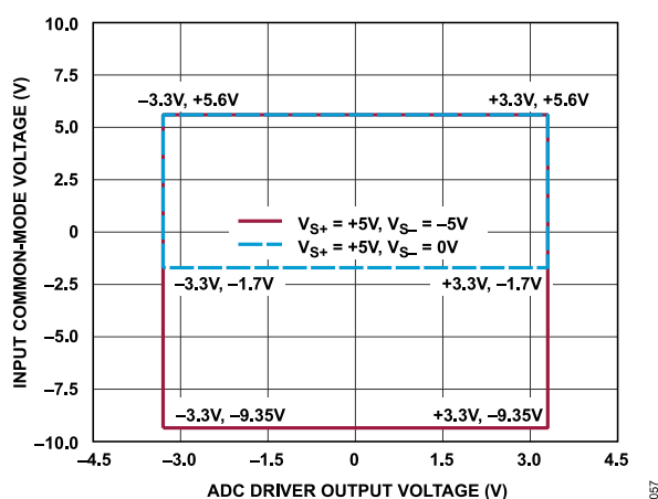
Figure 57. Input Common-Mode Voltage vs. ADC Driver Output, Gain = 1.0, \pm 3.3 V Differential Input
