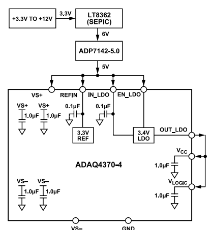
Figure 65. ADAQ4370-4 Power-Supply Recommendations
