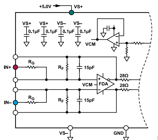
Figure 58. ADAQ4370-4 Configured at Fully-Differential Inputs
