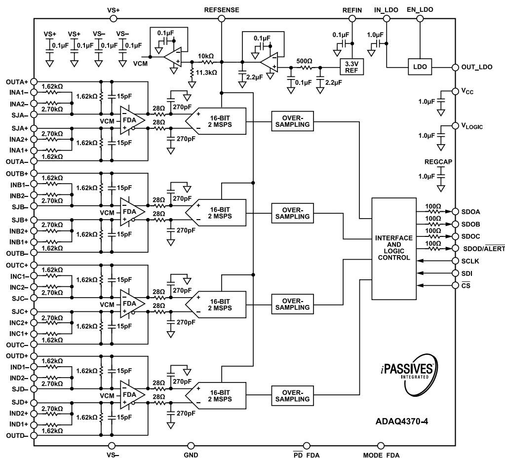
Figure 46. ADAQ4370-4 μModule Simplified Block Diagram
