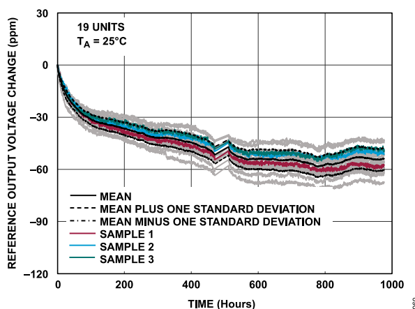
Figure 61. ADAQ4370-4 Internal-Reference Long-Term Drift
