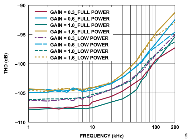
Figure 35. THD vs. Frequency
