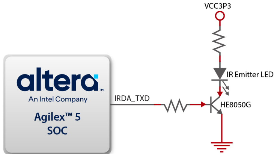
Figure 3-29 Connection between the FPGA and IR emitter LED
