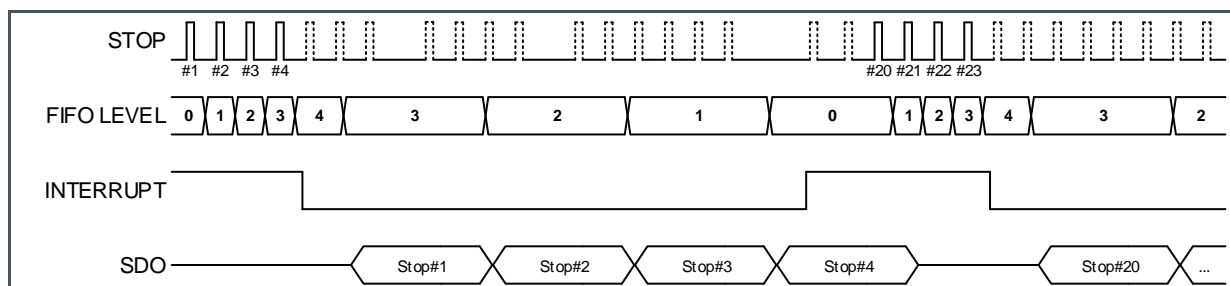
Figure 54: BLOCKWISE_FIFO_READ
