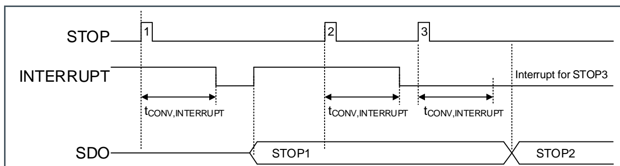
Figure 49: Conversion Latency
