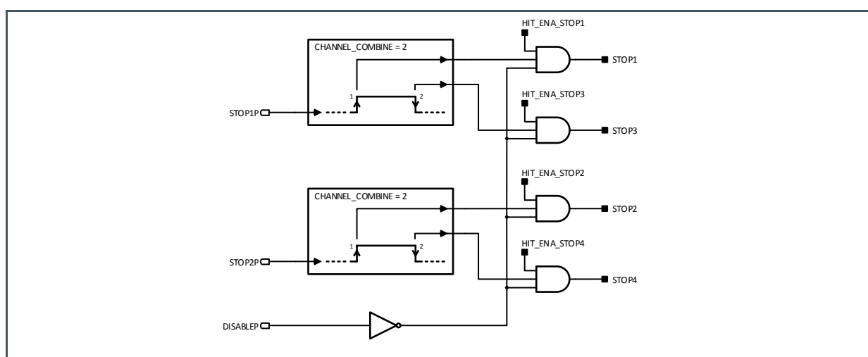
Figure 38: Channel Combination Pulse Width Measurement
