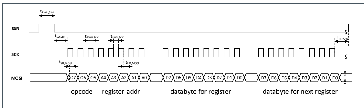
Figure 13: Write and Incremental Write
