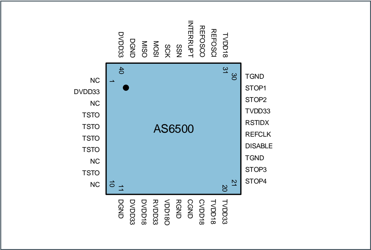
Figure 3: AS6500 QFN40
