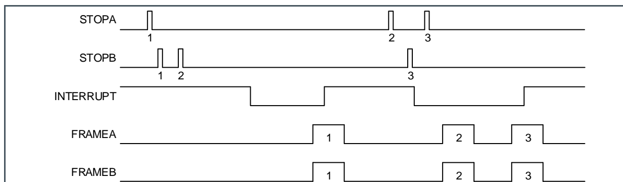
Figure 55: COMMON_FIFO_READ
