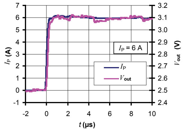
Figure 4: Step response
