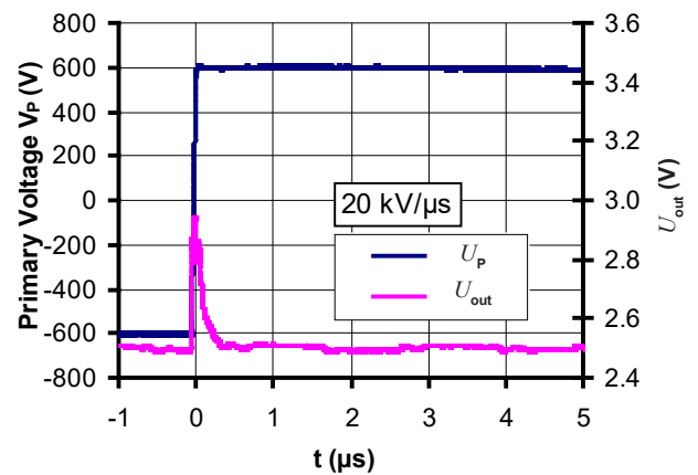
Figure 18: dv/dt
