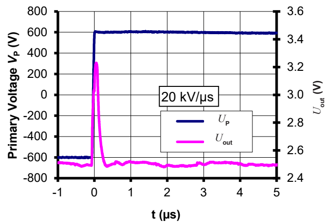
Figure 12: dv/dt
